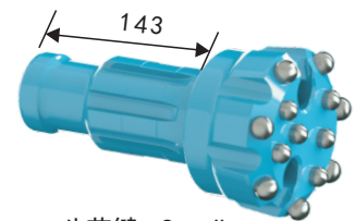
八花键 8 splines
